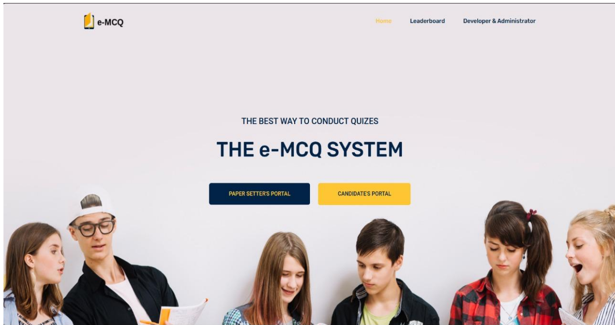
Screenshot 1: Homepage
